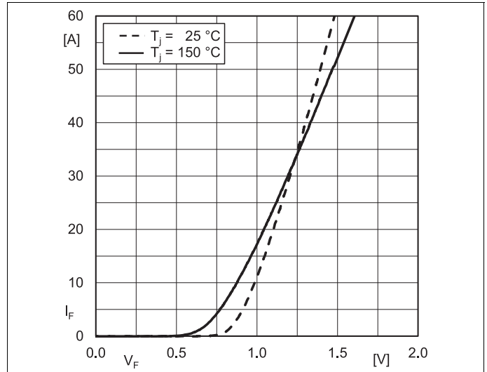
Fig. 14: Typ. Rect. diode forward charact., incl. R_{CC'+EE}
